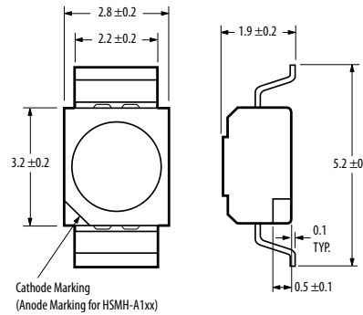
PLCC-2 Reverse Mount
