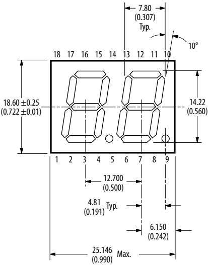
14.2 mm (0.56”) Dual Digit Displays Package Dimension
