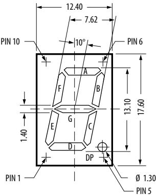
13.1mm (0.52”) Single Digit Displays Package Dimension
