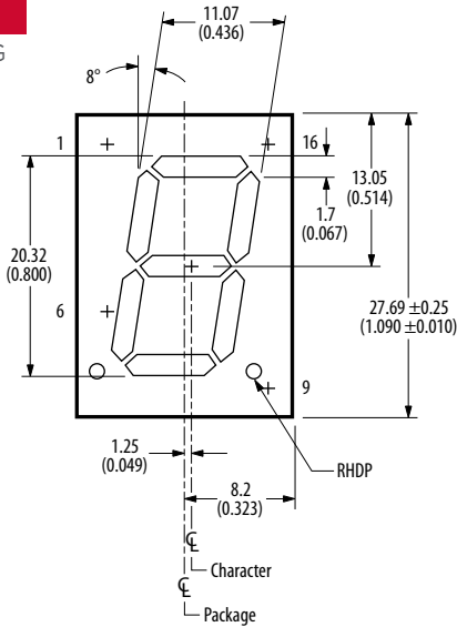
20 mm (0.8”) Single Digit Displays Package Dimension
